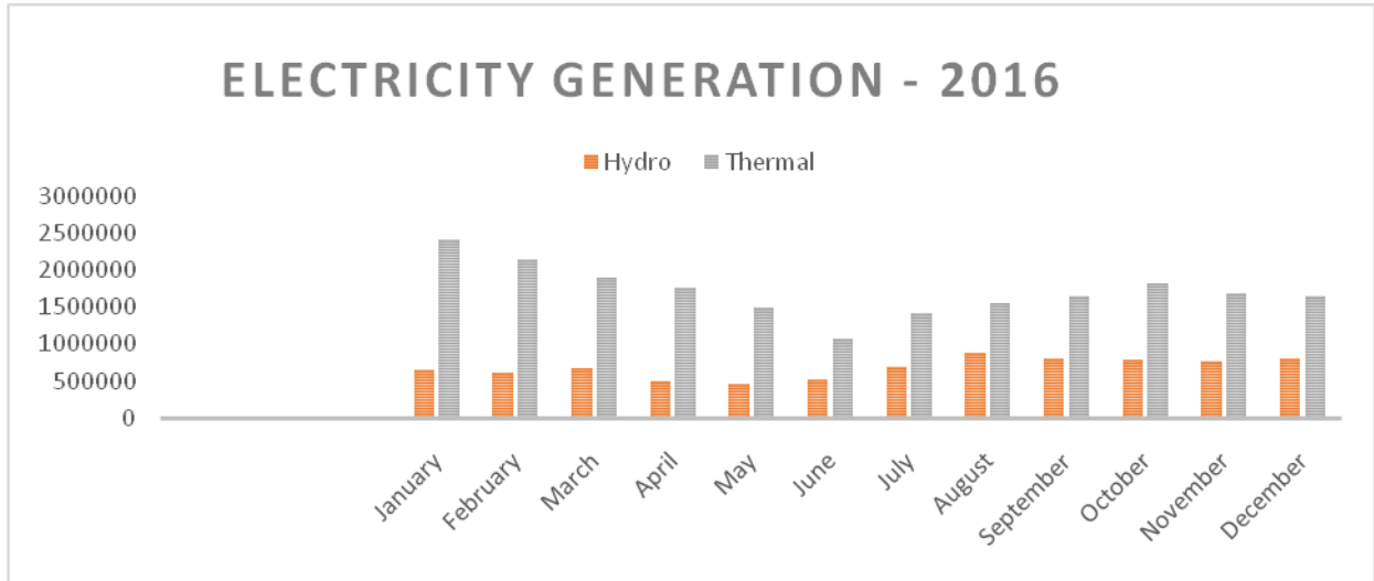
CHART 13.2: ELECTRICITY GENERATION BY PLANTS
