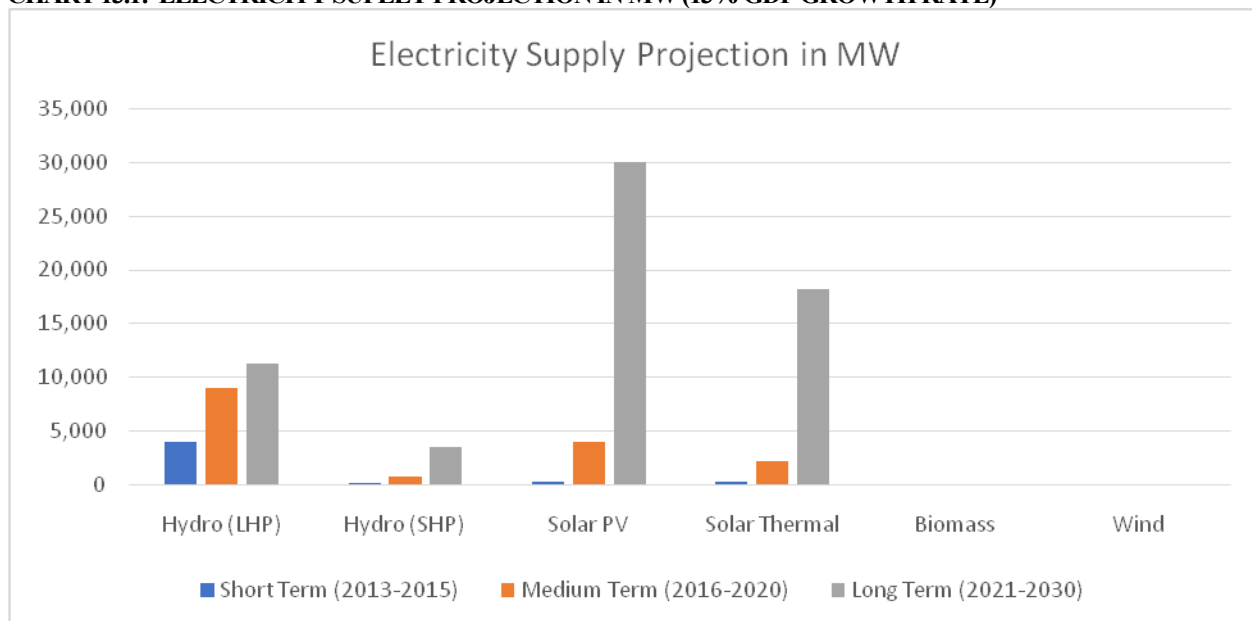
CHART 13.1: ELECTRICITY SUPPLY PROJECTION IN MW (13% GDP GROWTH RATE)
