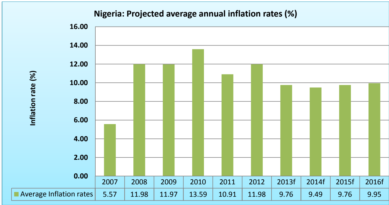
Figure 7: Inflation Projections (2013-2016)
