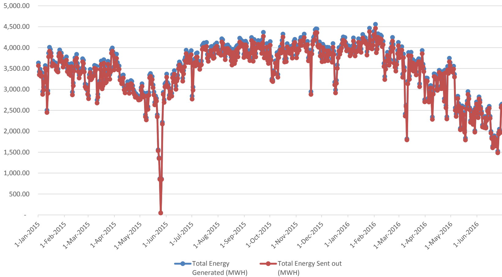
Total Energy Generated and Sent out (MWH/H) Jan 2015 to June 2016
